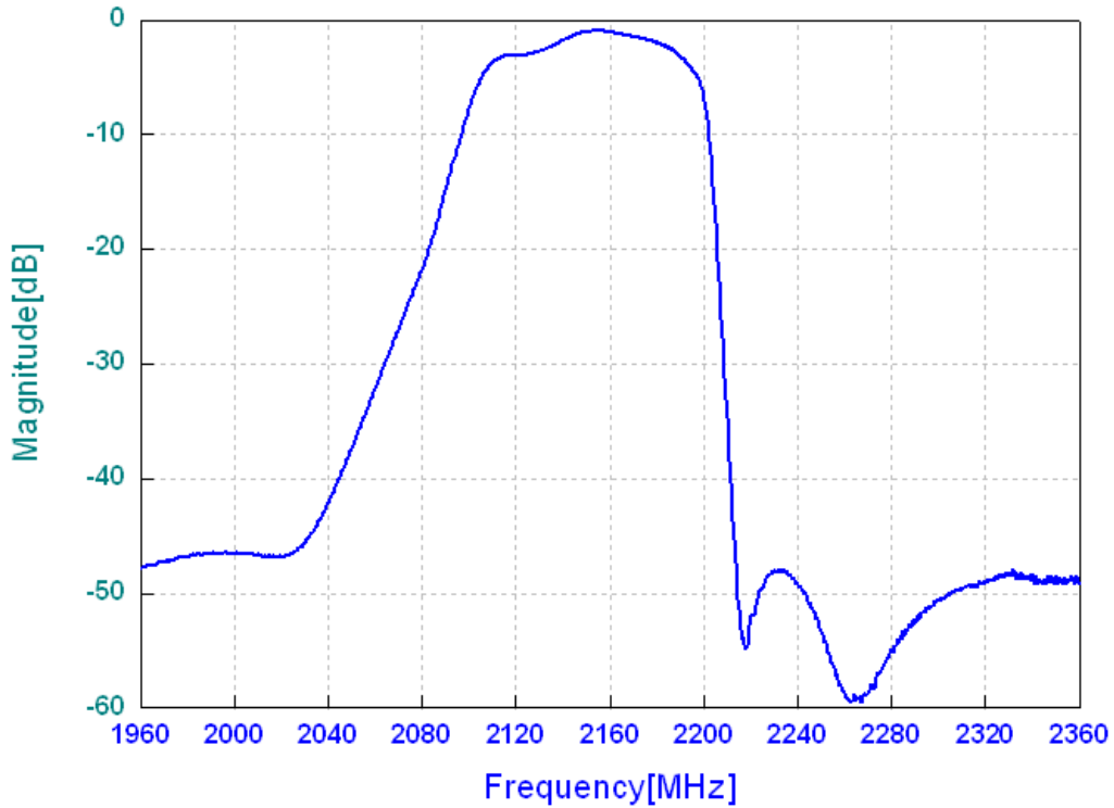
Frequency Response
